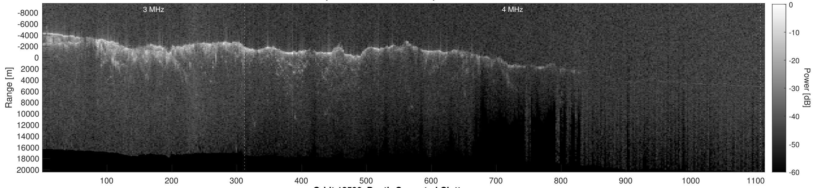
Orbit 12590, Depth-Corrected Cluttergram
