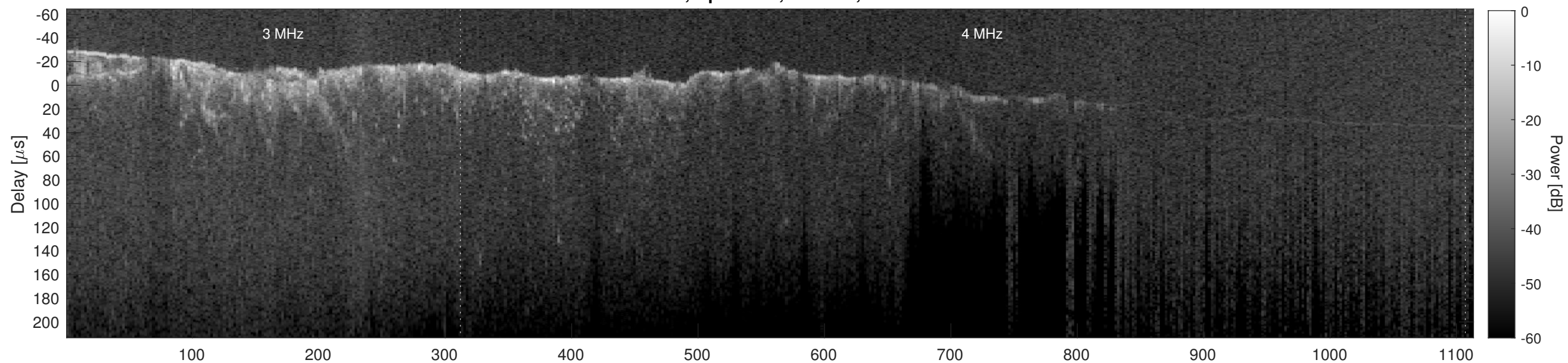
Orbit 12590, Cluttergram
