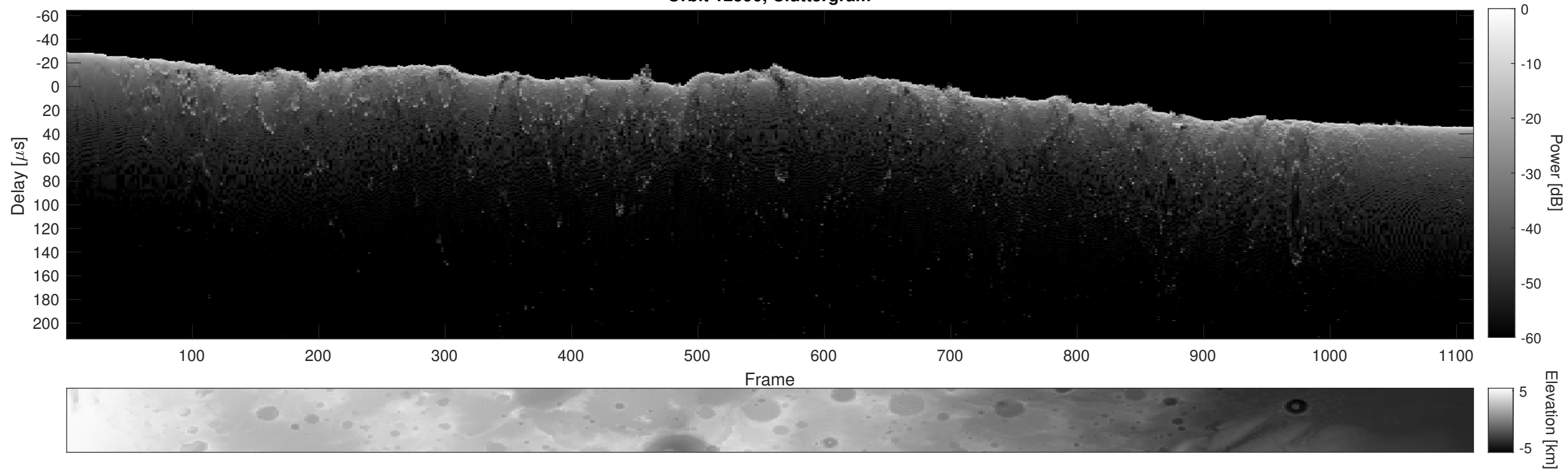
Orbit 12590, Cluttergram
