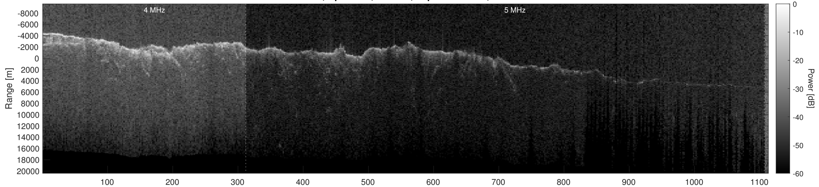
Orbit 12590, Optimized, Window, Depth-Corrected, Channel 2
