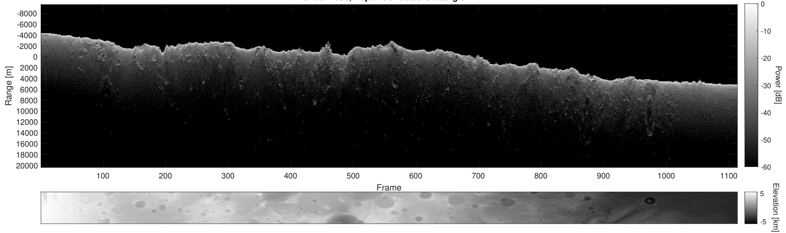
Orbit 12590, Depth-Corrected Cluttergram
