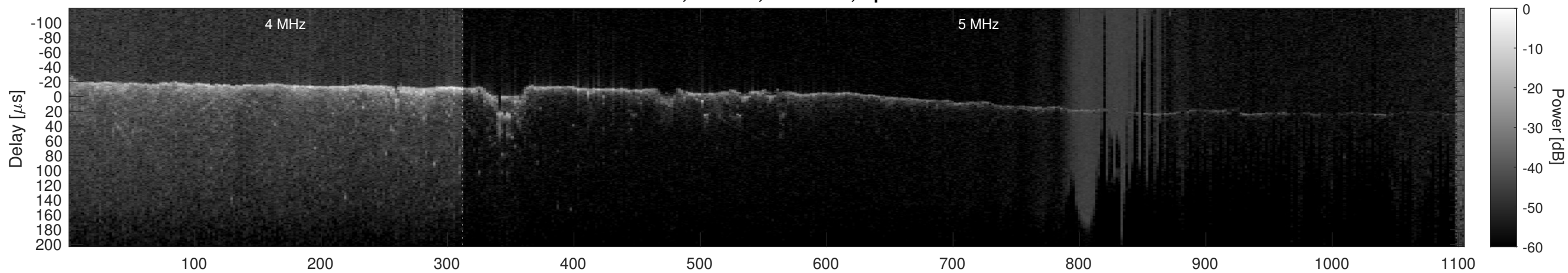
Orbit 12592, Cluttergram
