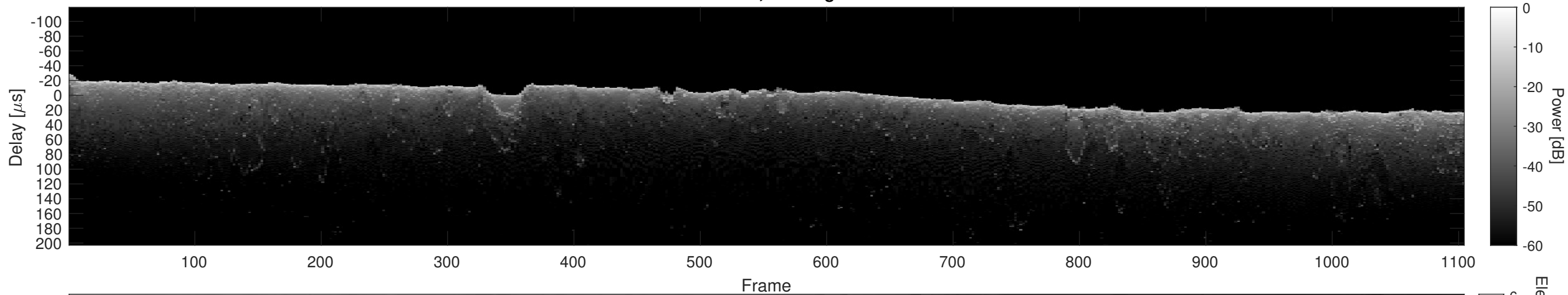
Orbit 12592, Cluttergram
