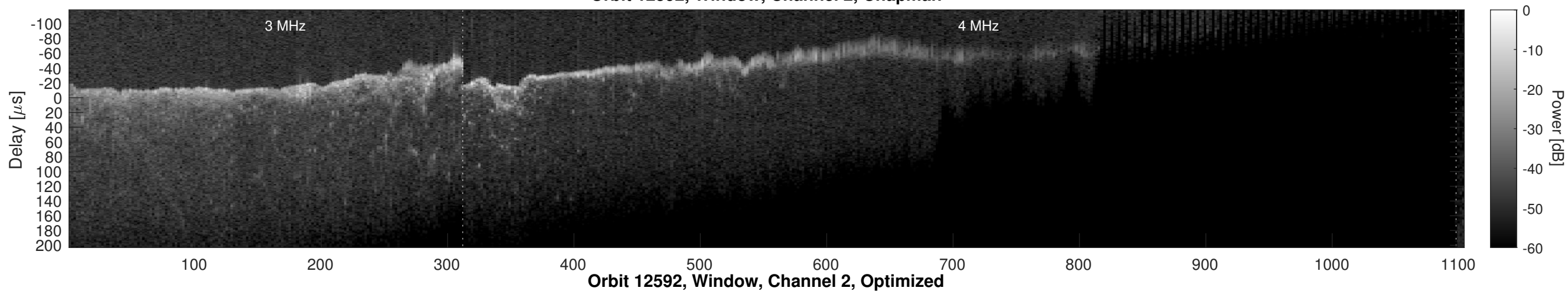
Orbit 12592, Window, Channel 2, Chapman
