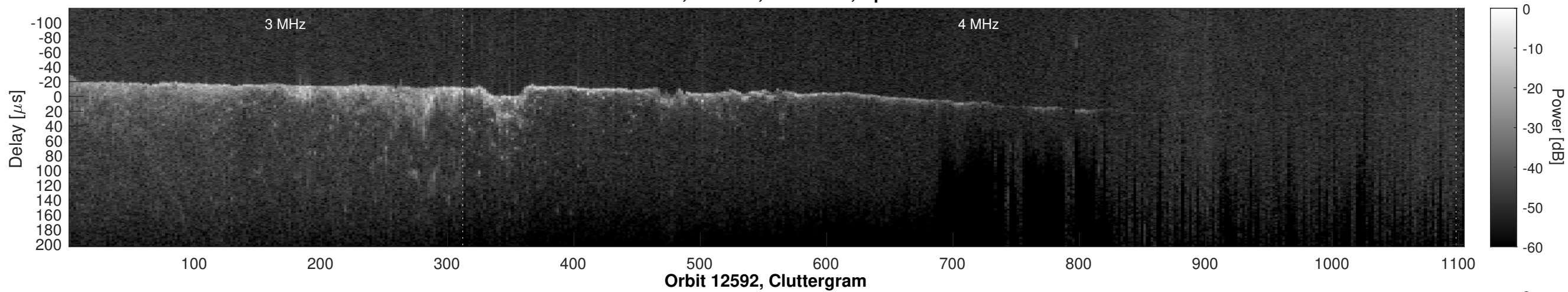
Orbit 12592, Window, Channel 2, Optimized
