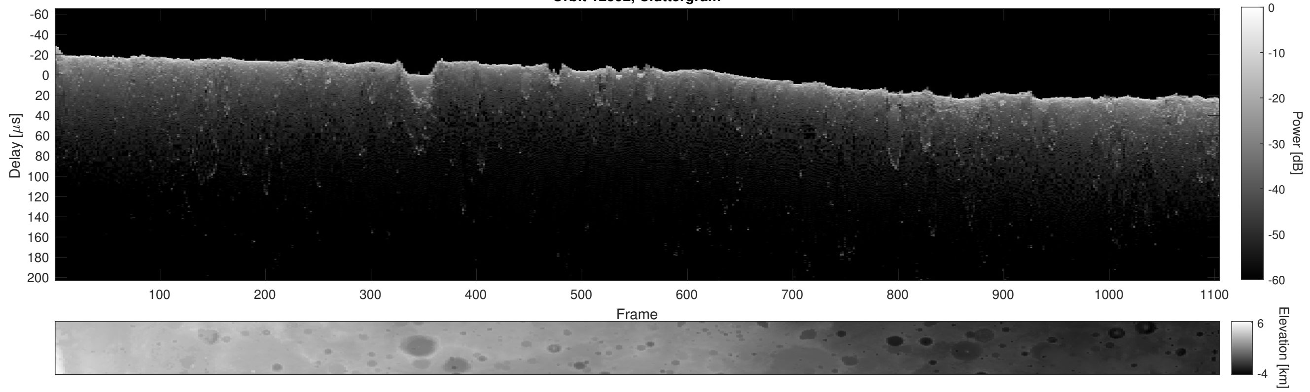
Orbit 12592, Cluttergram
