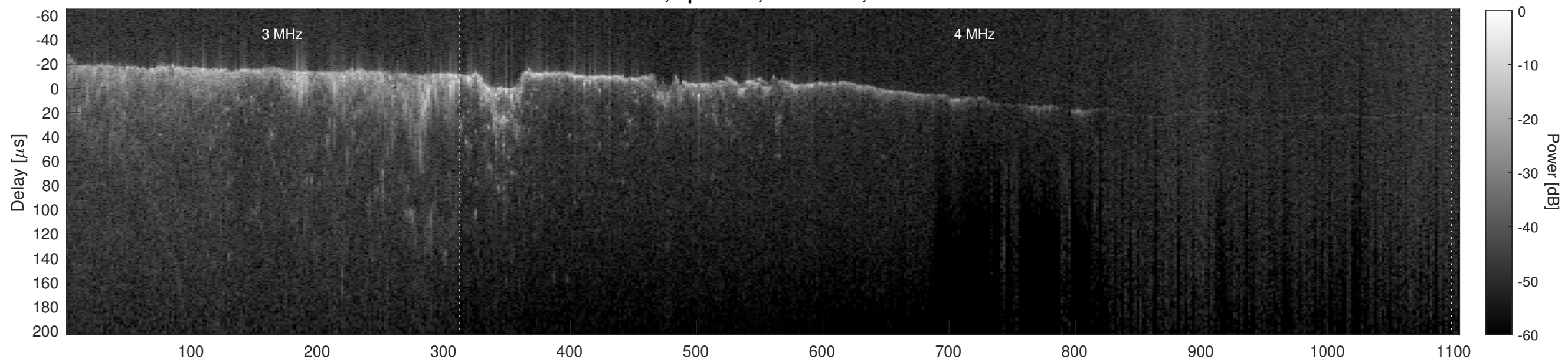
Orbit 12592, Cluttergram
