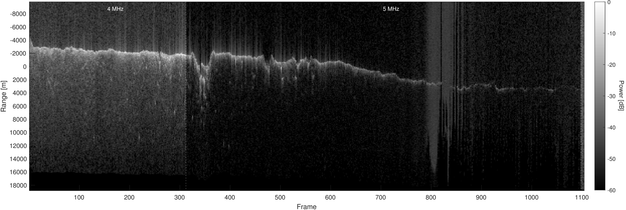
Orbit 12592, Optimized, No Window, Depth-Corrected, Channel 2
