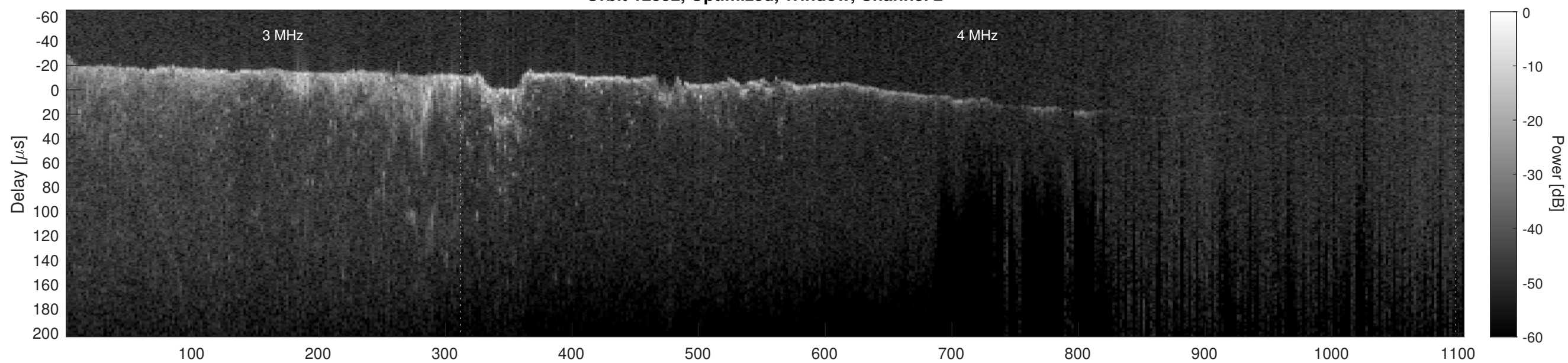
Orbit 12592, Cluttergram
