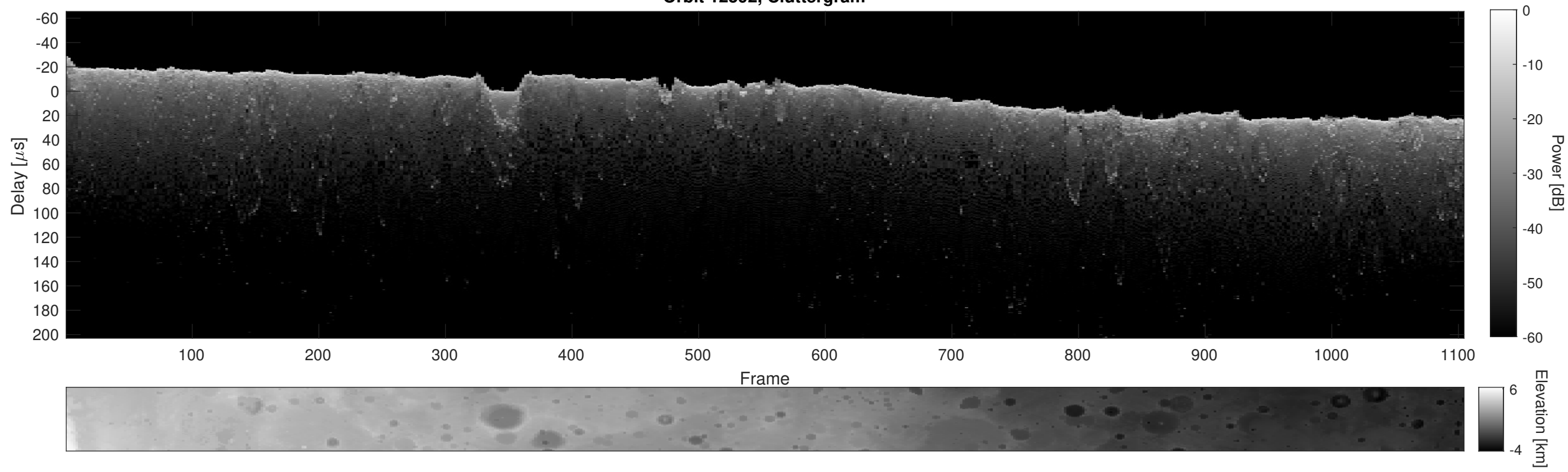
Orbit 12592, Cluttergram
