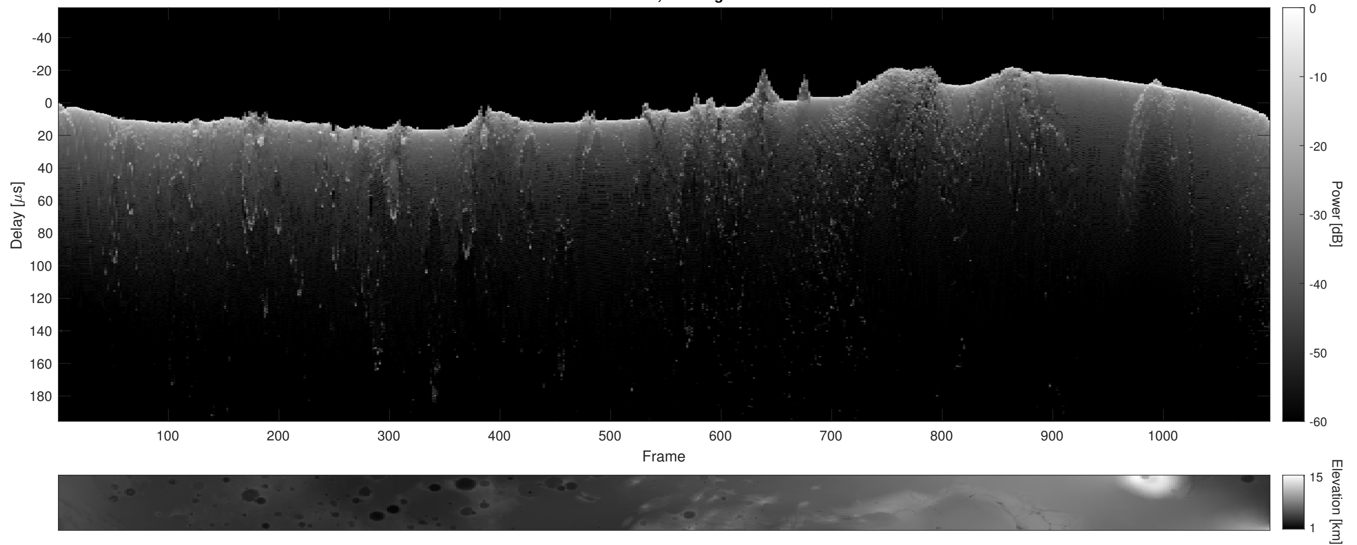
Orbit 12593, Cluttergram
