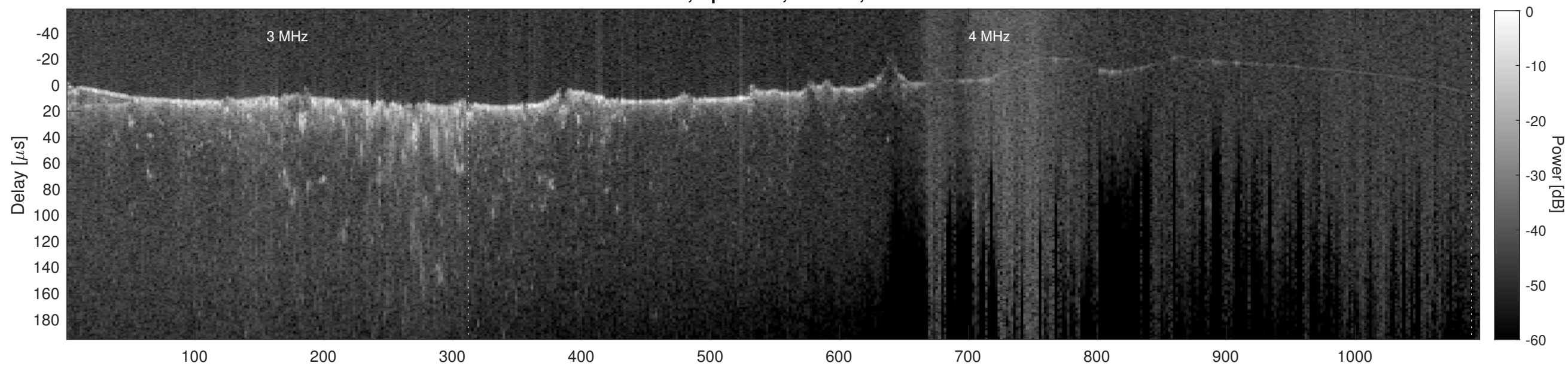
Orbit 12593, Cluttergram
