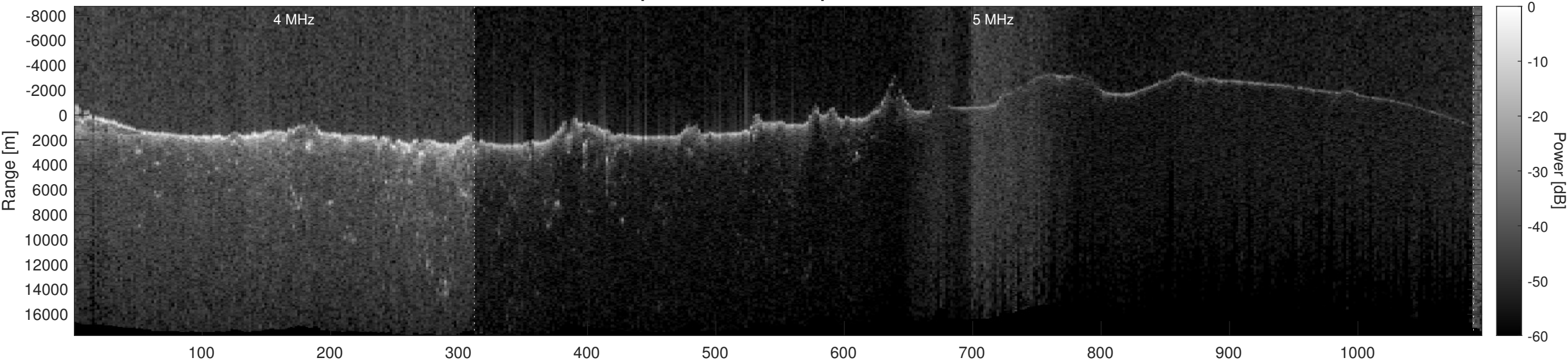
Orbit 12593, Optimized, Window, Depth-Corrected, Channel 2
