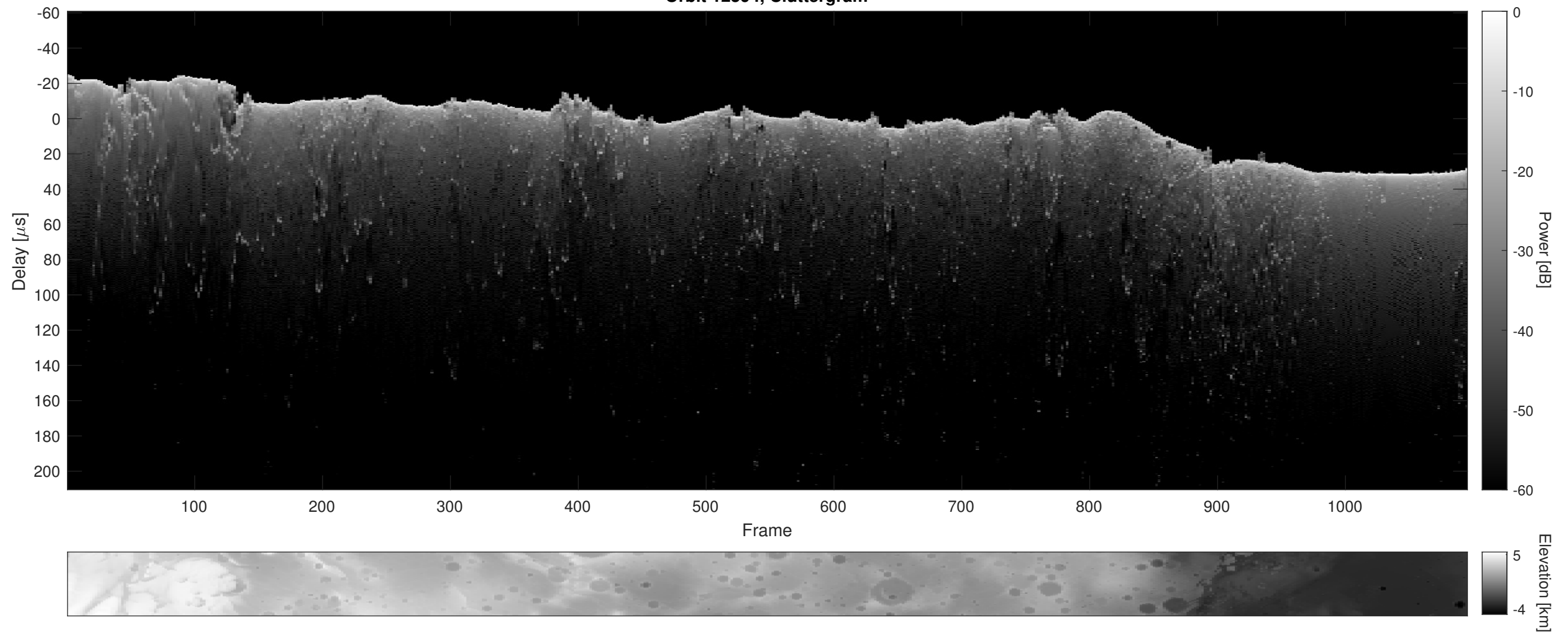
Orbit 12594, Cluttergram
