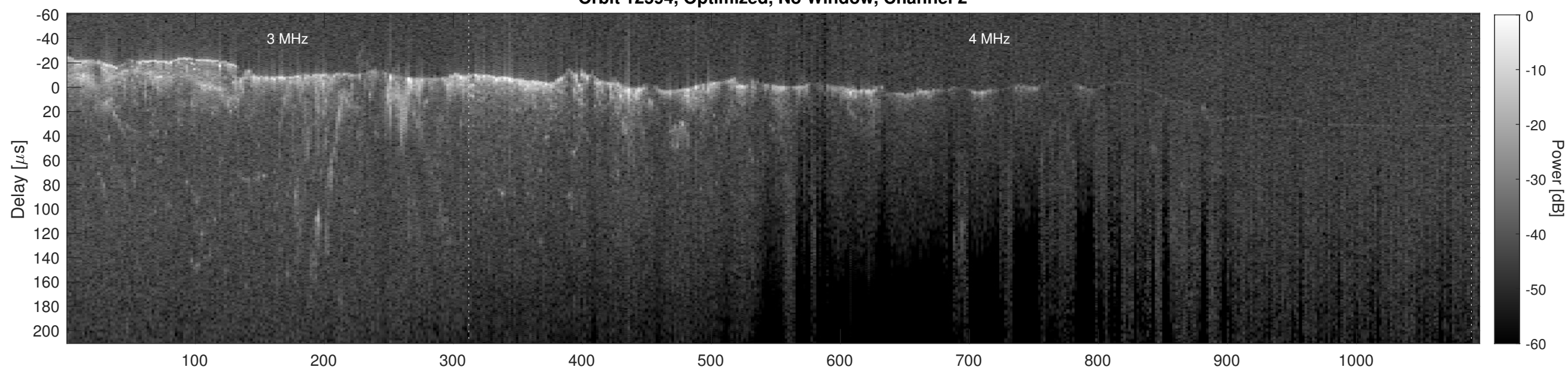
Orbit 12594, Cluttergram
