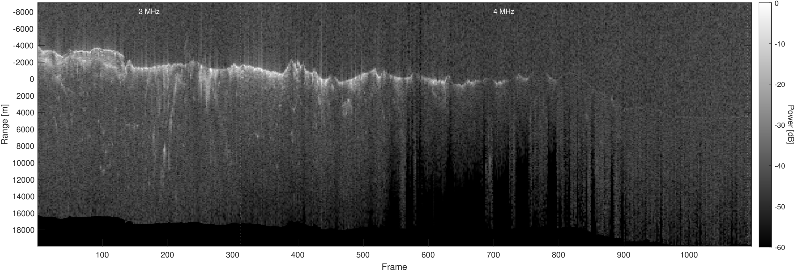
Orbit 12594, Optimized, No Window, Depth-Corrected, Channel 2
