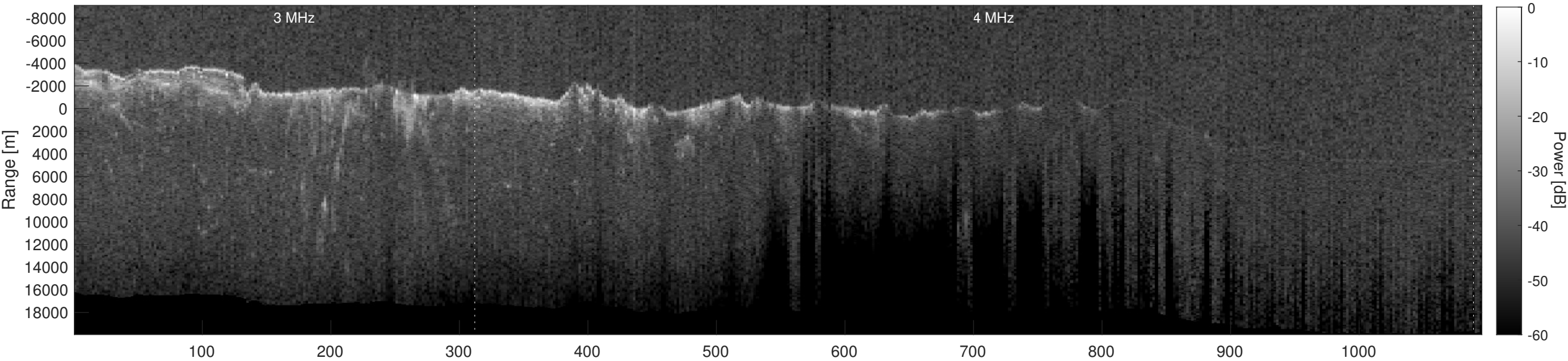
Orbit 12594, Depth-Corrected Cluttergram
