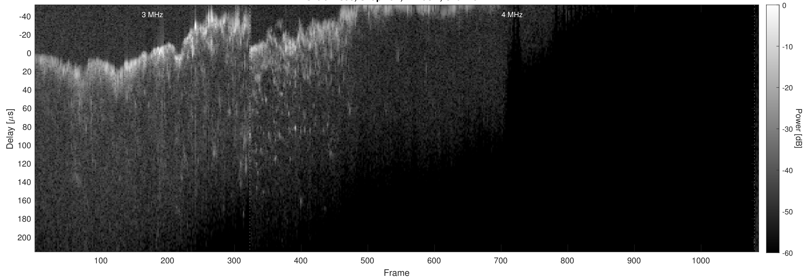
Orbit 12596, Chapman, Window, Channel 2
