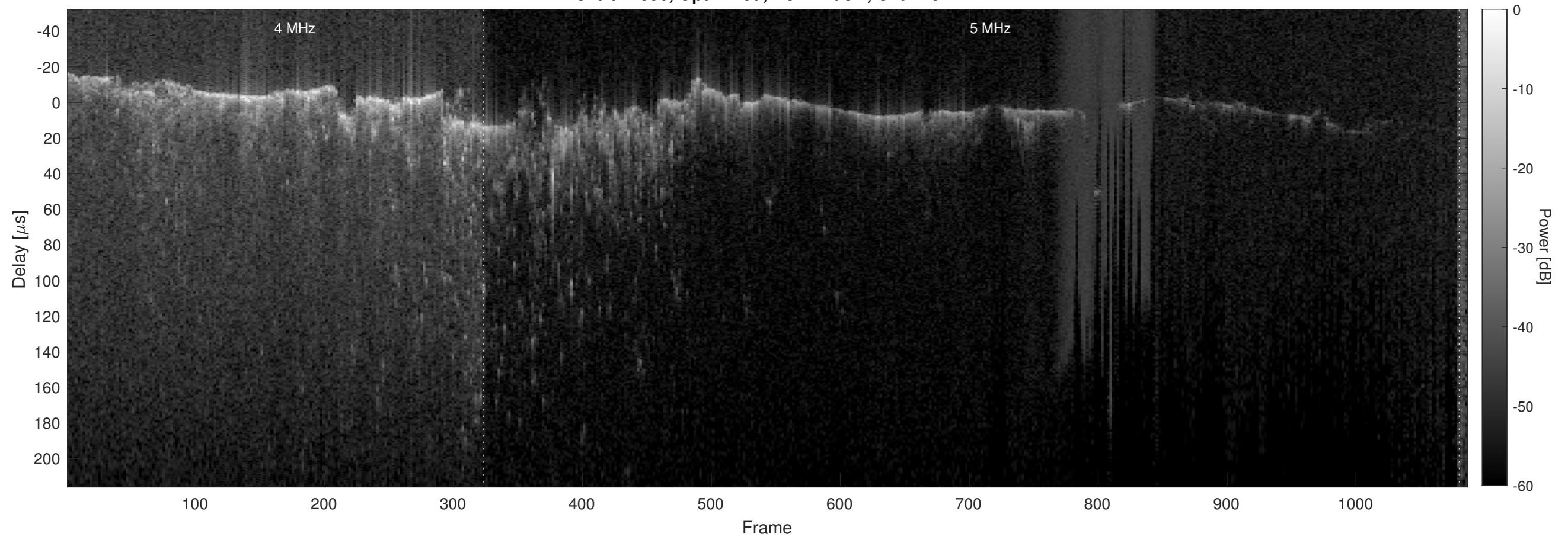
Orbit 12596, Optimized, No Window, Channel 2
