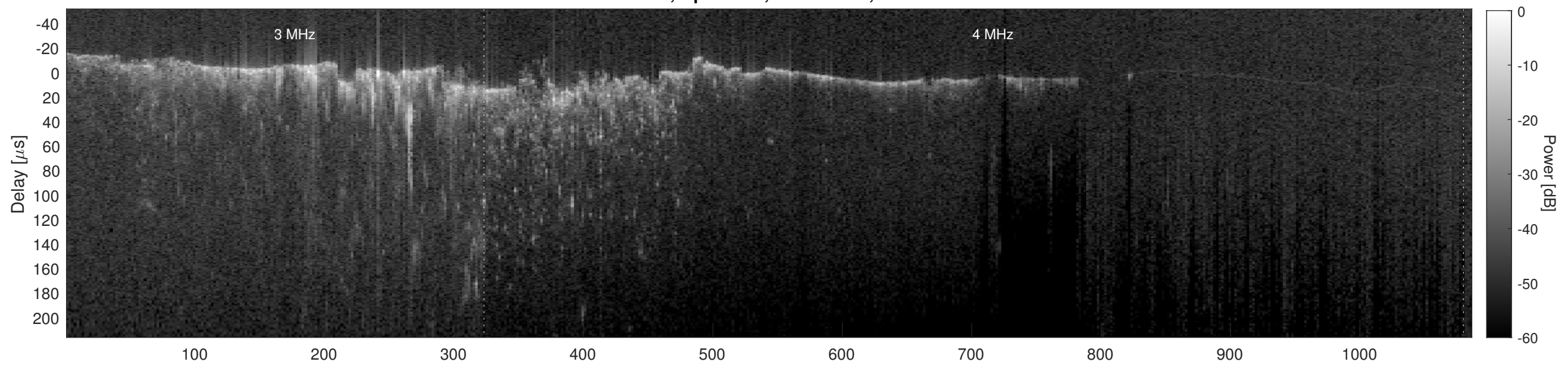
Orbit 12596, Cluttergram
