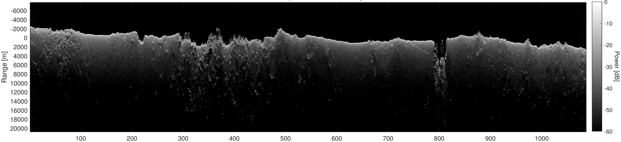
Orbit 12596, Depth-Corrected Cluttergram
