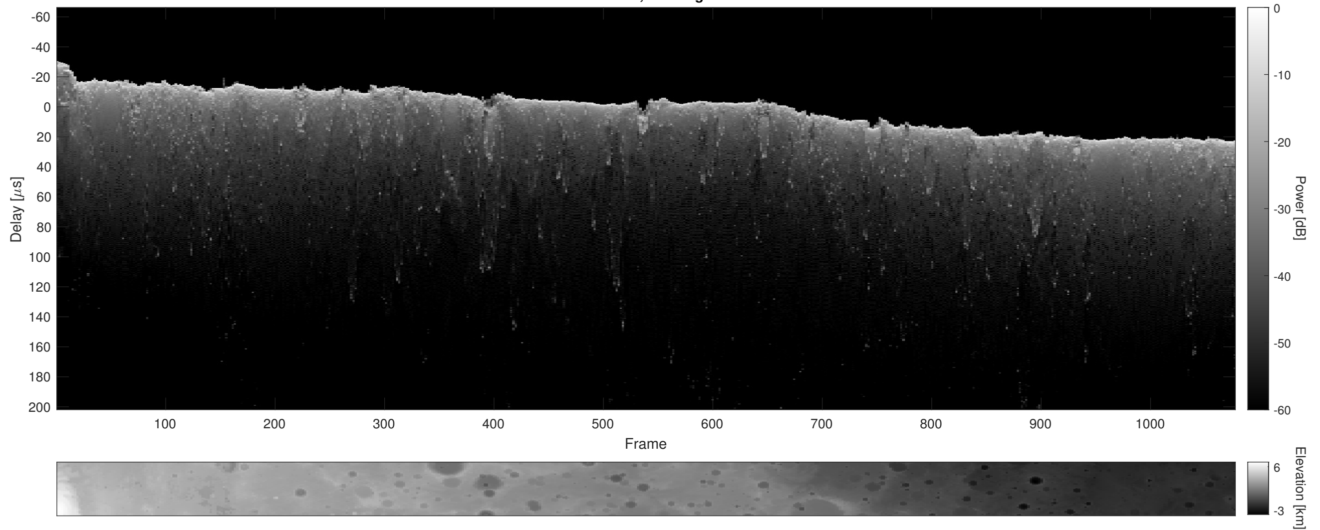
Orbit 12599, Cluttergram
