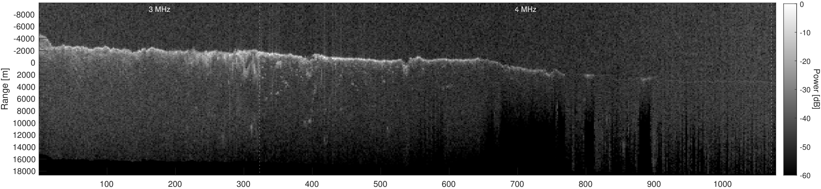
Orbit 12599, Depth-Corrected Cluttergram
