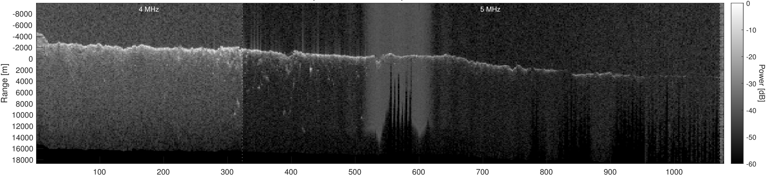
Orbit 12599, Optimized, Window, Depth-Corrected, Channel 2
