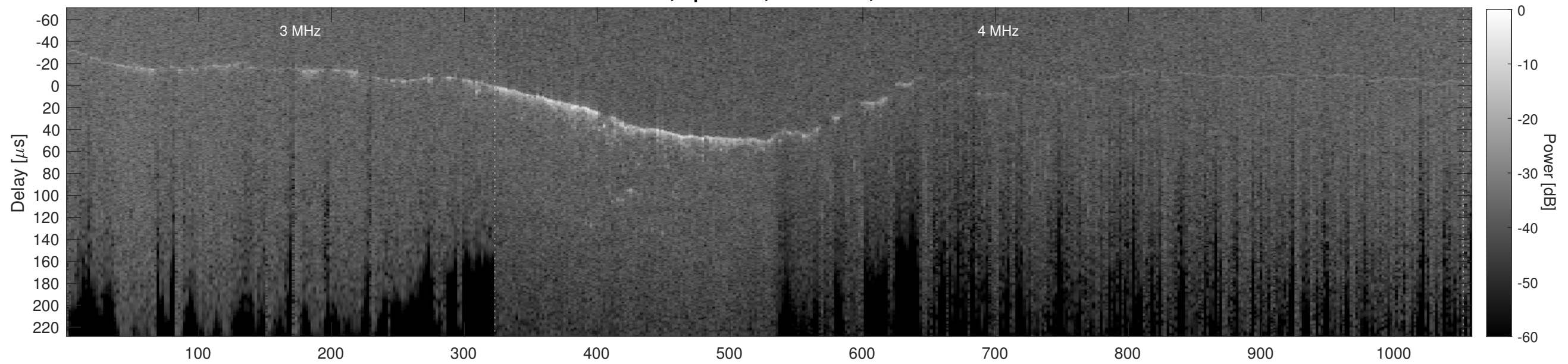
Orbit 12602, Cluttergram
