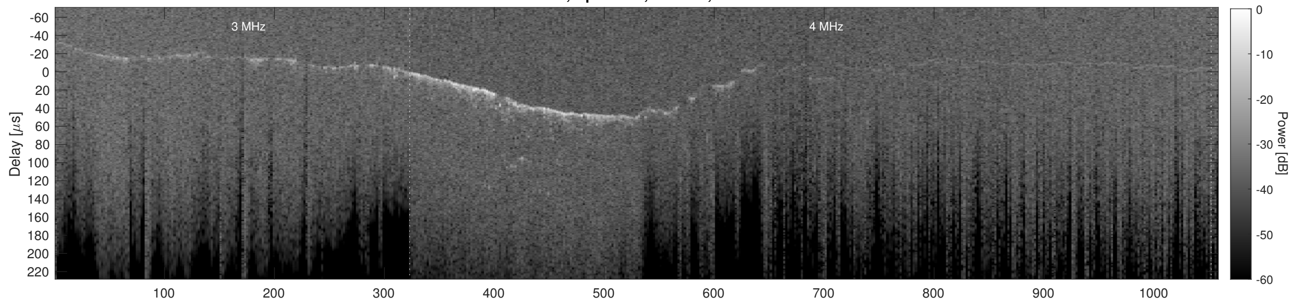
Orbit 12602, Cluttergram
