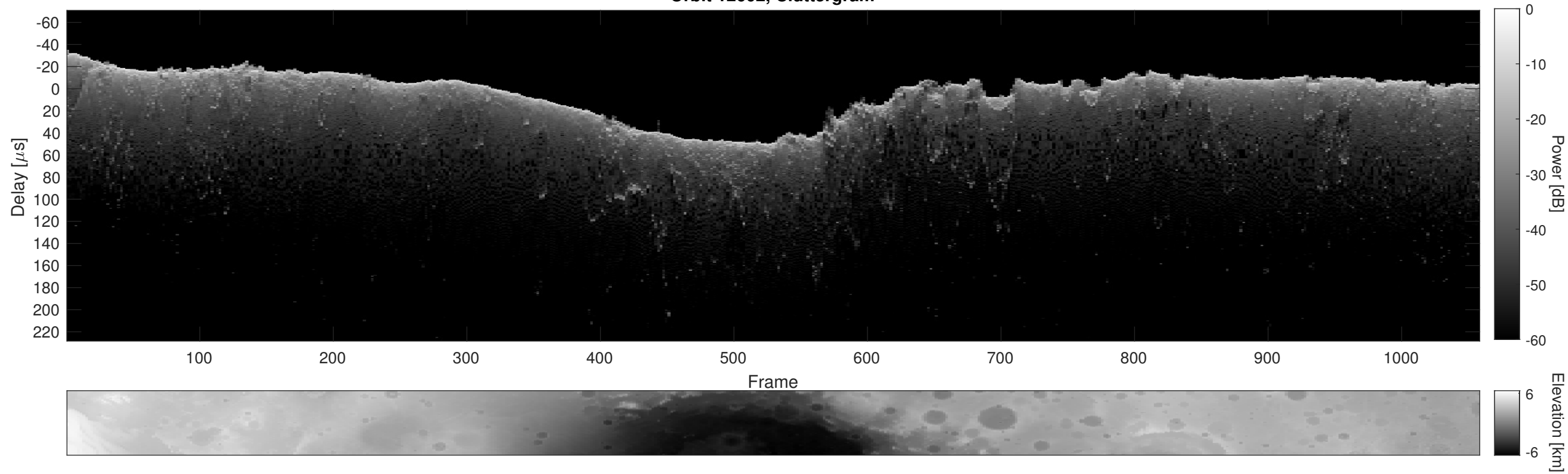
Orbit 12602, Cluttergram
