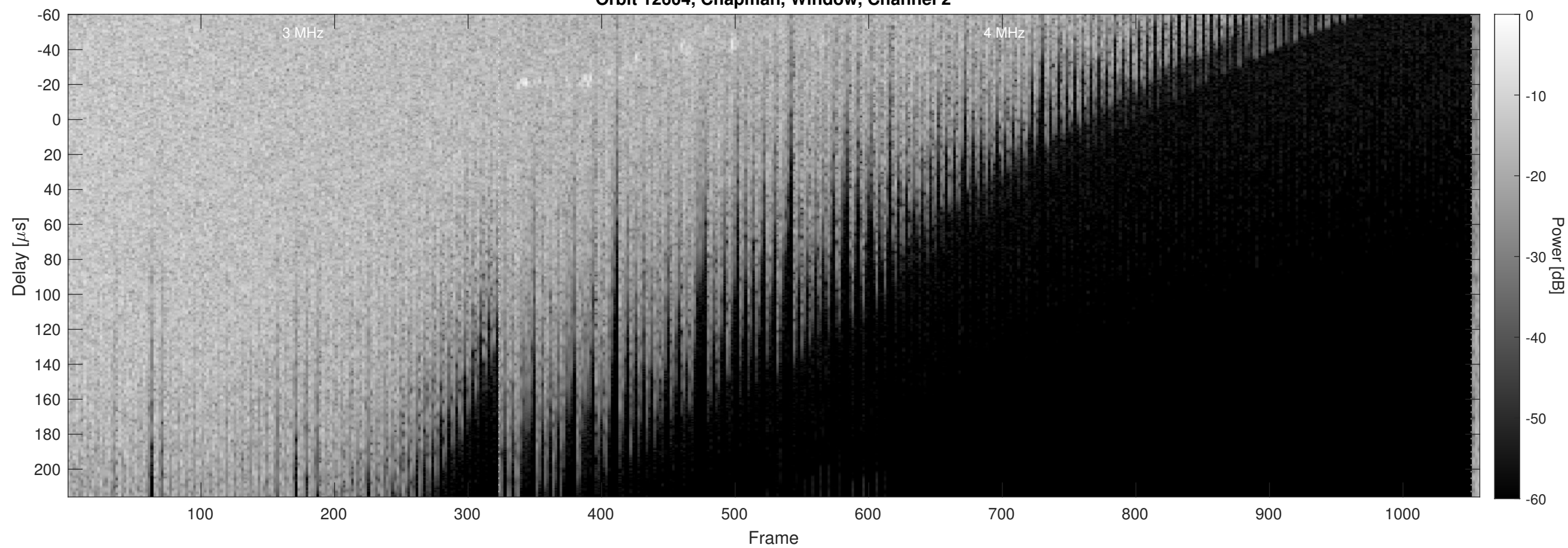
Orbit 12604, Chapman, Window, Channel 2
