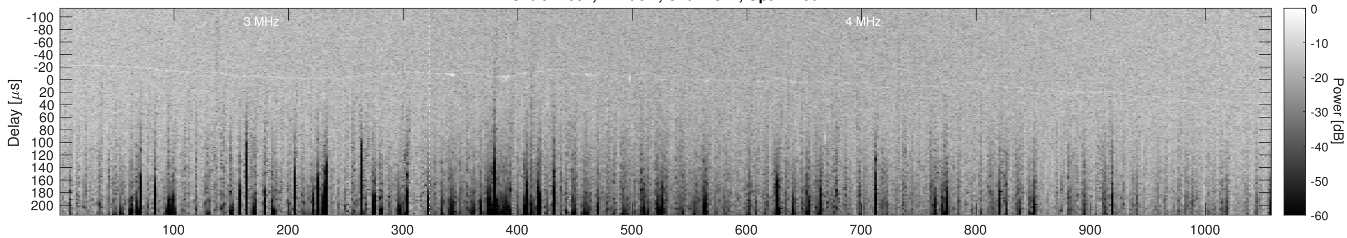
Orbit 12604, Cluttergram
