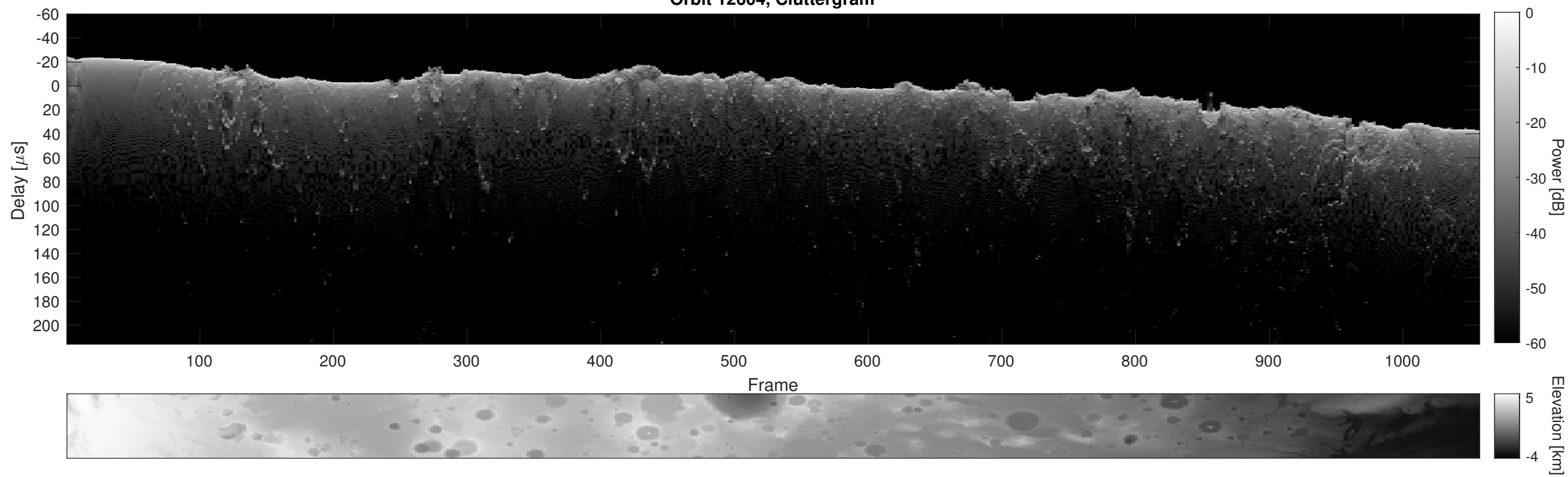
Orbit 12604, Cluttergram
