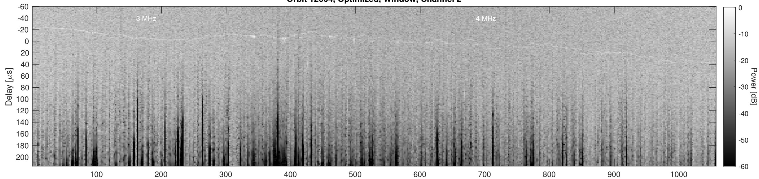
Orbit 12604, Cluttergram
