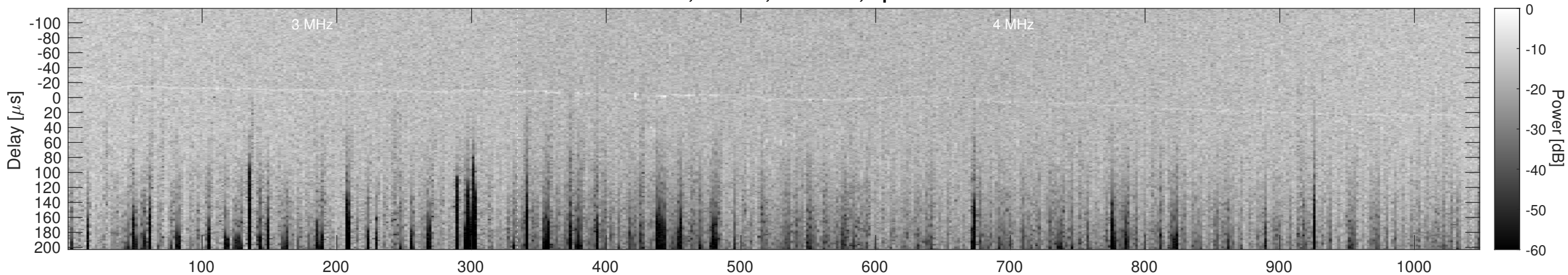
Orbit 12606, Cluttergram
