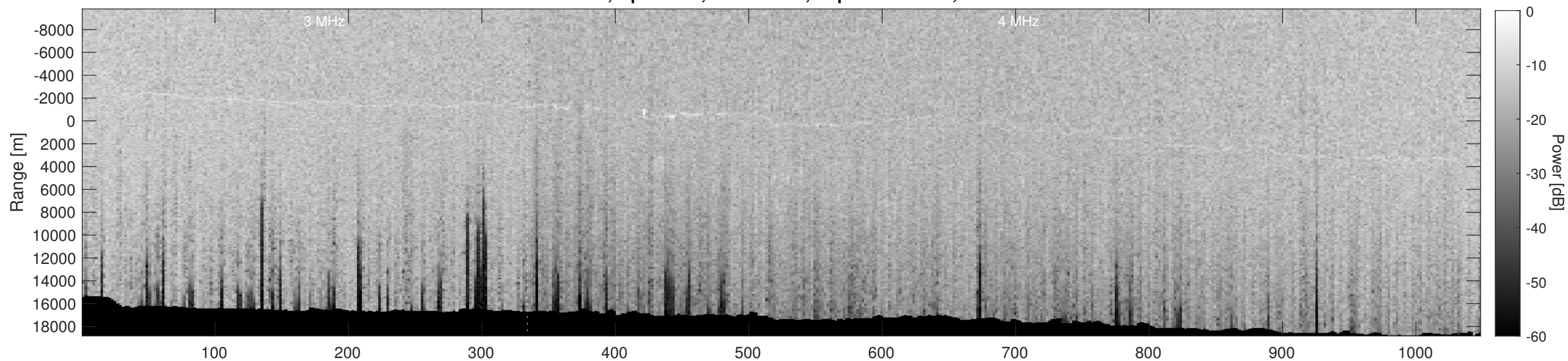
Orbit 12606, Depth-Corrected Cluttergram
