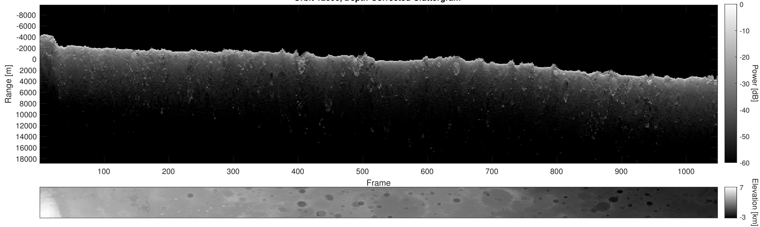
Orbit 12606, Depth-Corrected Cluttergram
