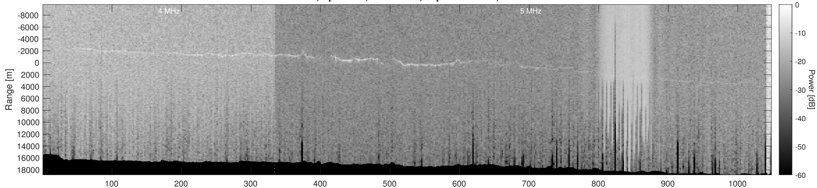
Orbit 12606, Optimized, No Window, Depth-Corrected, Channel 2
