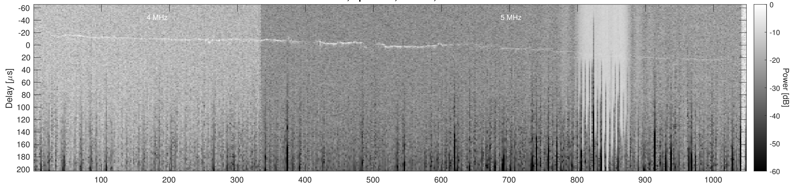
Orbit 12606, Optimized, Window, Channel 2
