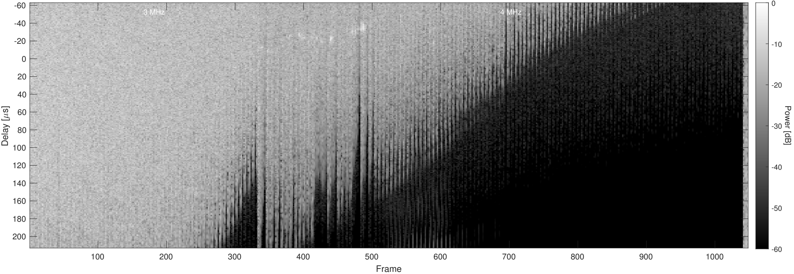
Orbit 12608, Chapman, No Window, Channel 2
