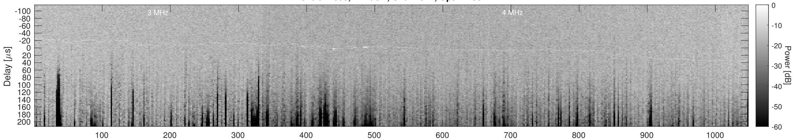
Orbit 12608, Cluttergram
