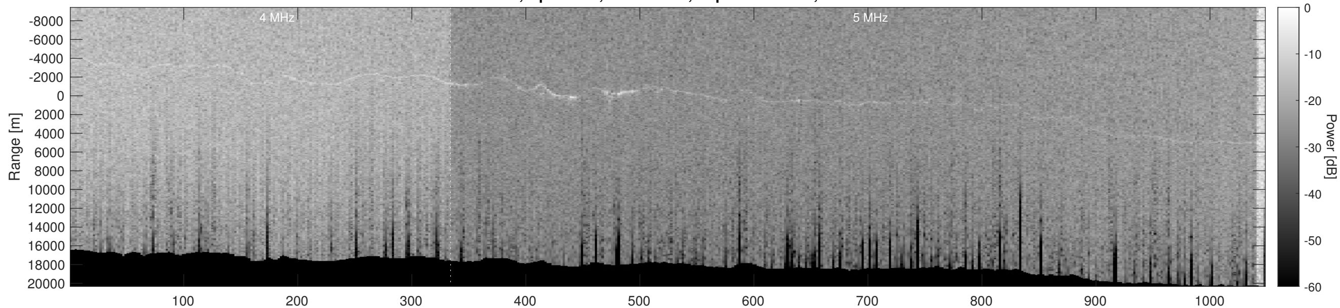
Orbit 12608, Optimized, No Window, Depth-Corrected, Channel 2
