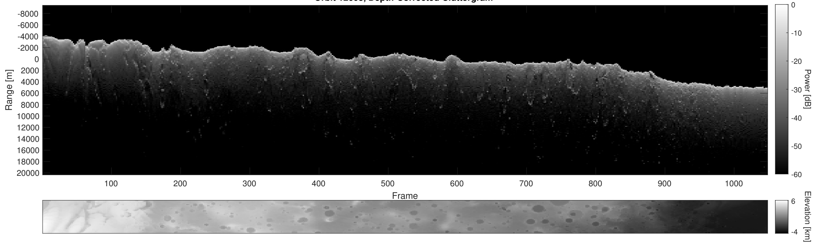
Orbit 12608, Depth-Corrected Cluttergram
