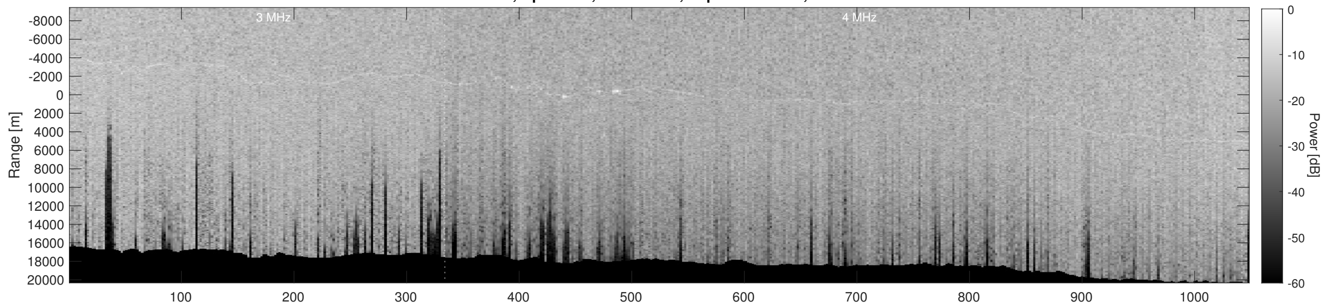
Orbit 12608, Depth-Corrected Cluttergram
