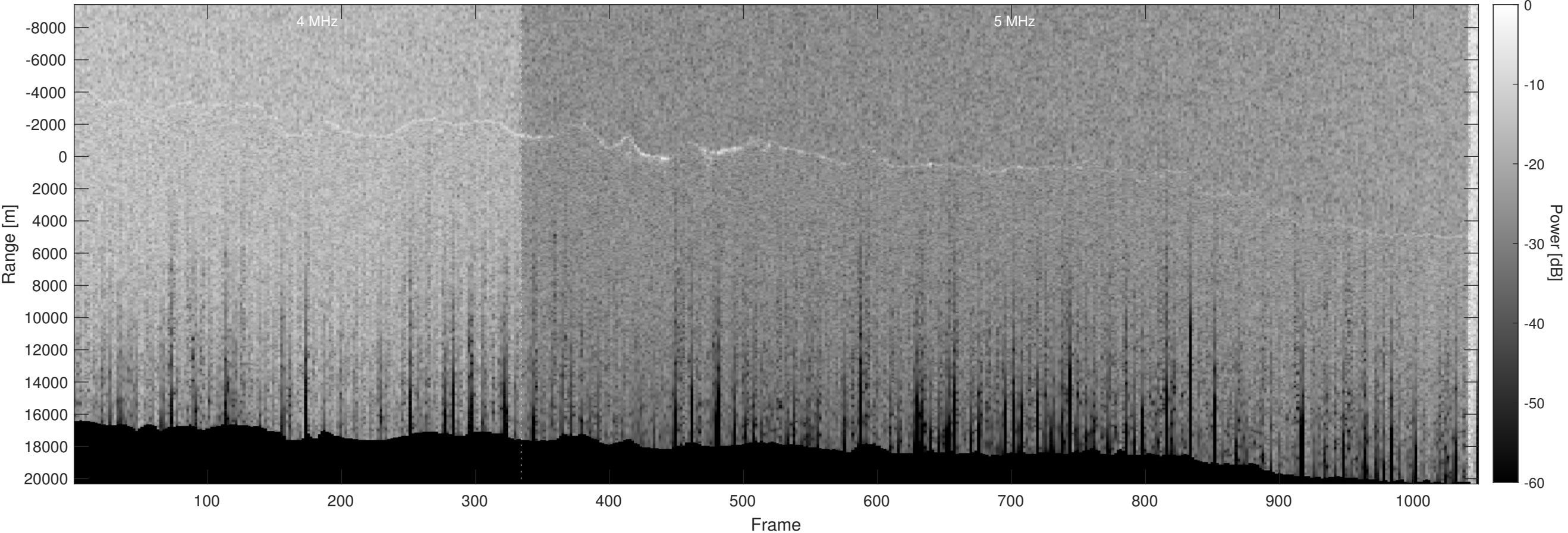
Orbit 12608, Optimized, Window, Depth-Corrected, Channel 2
