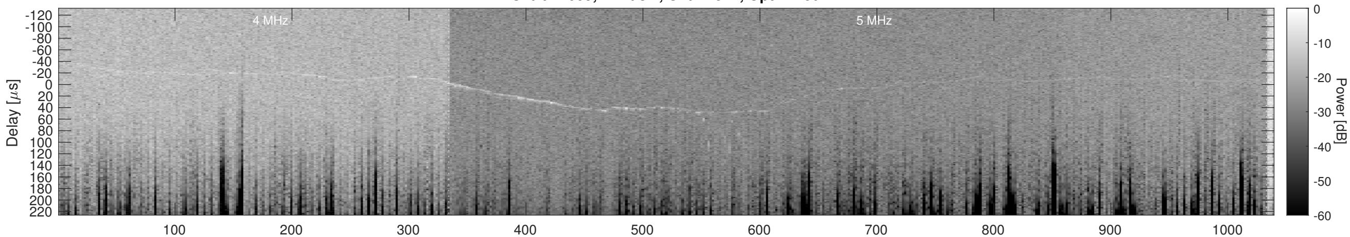
Orbit 12609, Cluttergram
