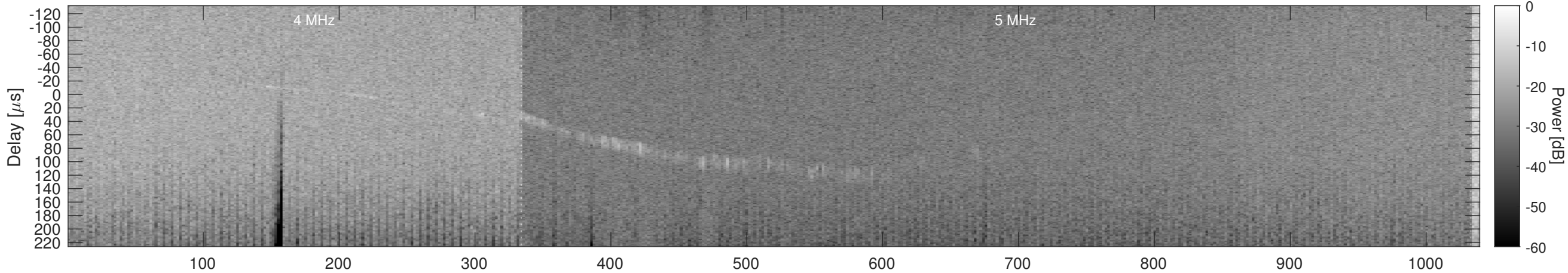
Orbit 12609, Window, Channel 1, Chapman
