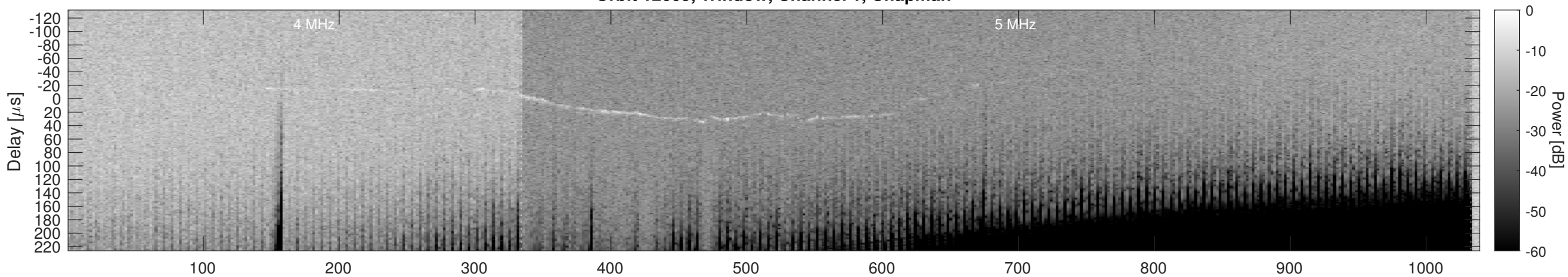
Orbit 12609, Window, Channel 1, Optimized
