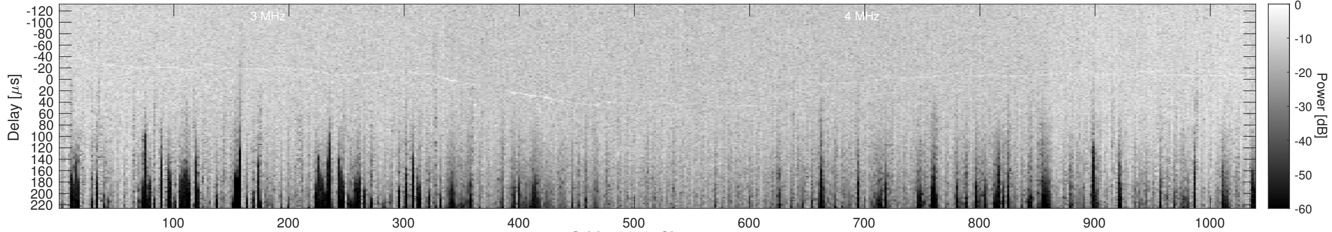
Orbit 12609, Cluttergram
