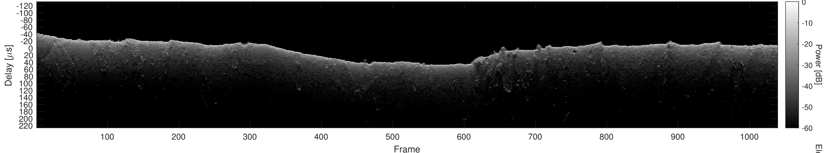
Orbit 12609, Cluttergram
