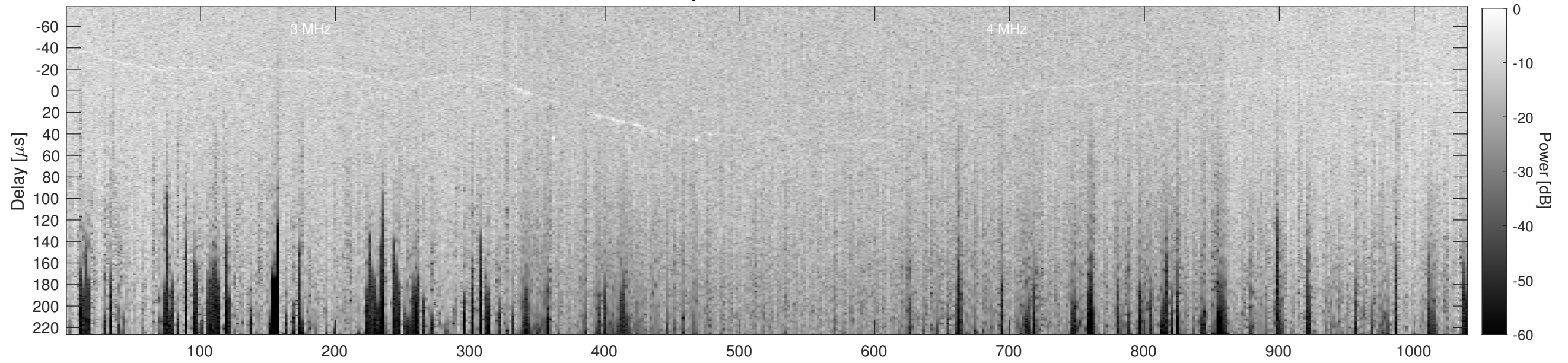
Orbit 12609, Cluttergram
