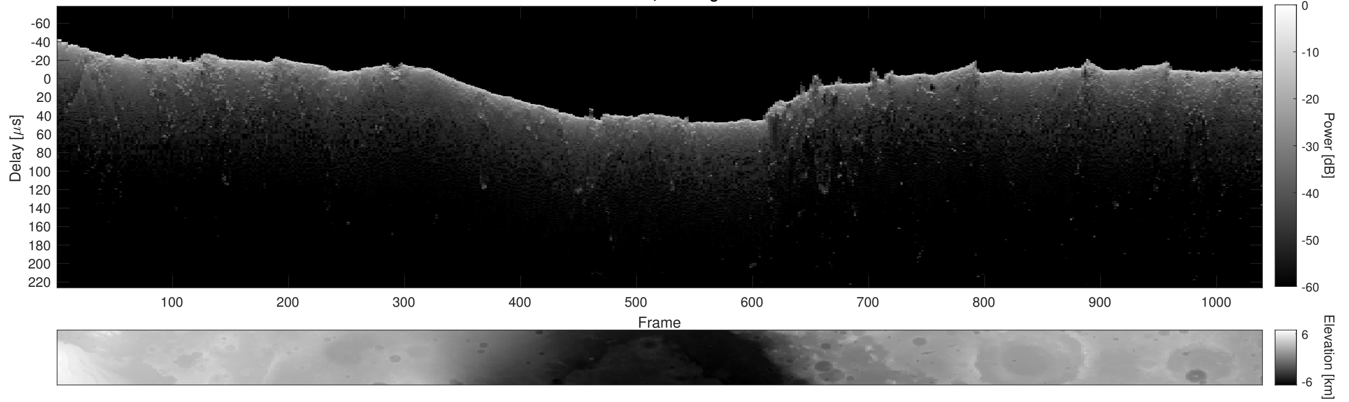
Orbit 12609, Cluttergram
