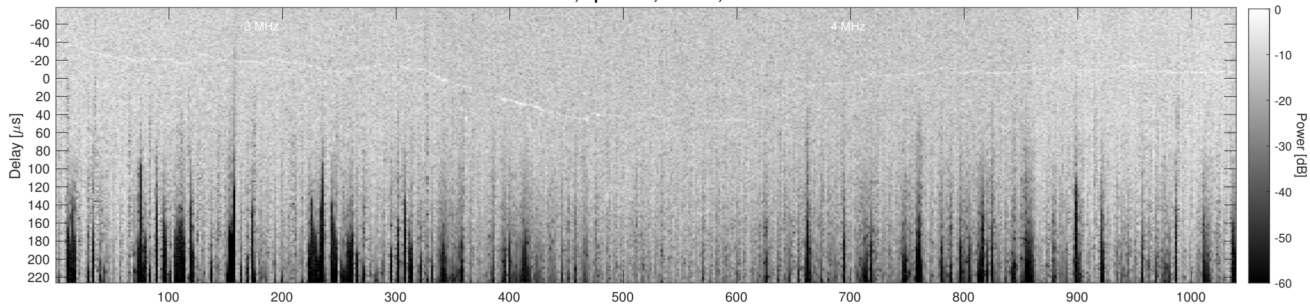
Orbit 12609, Cluttergram
