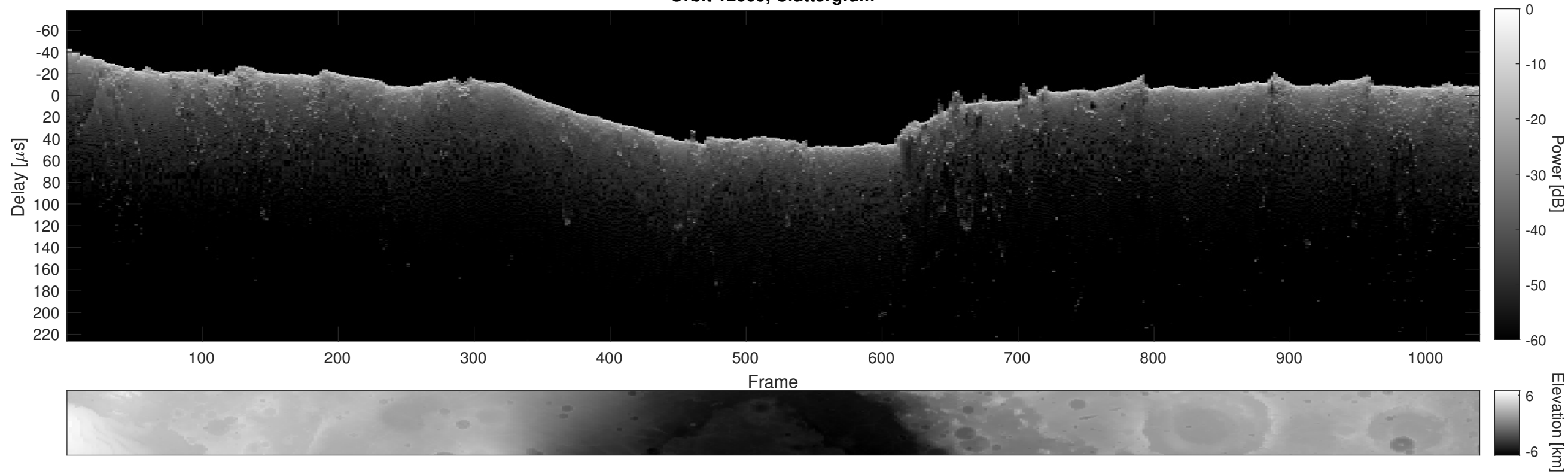
Orbit 12609, Cluttergram
