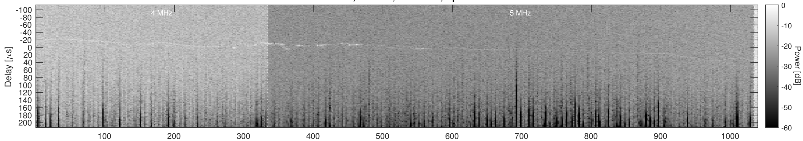
Orbit 12611, Cluttergram
