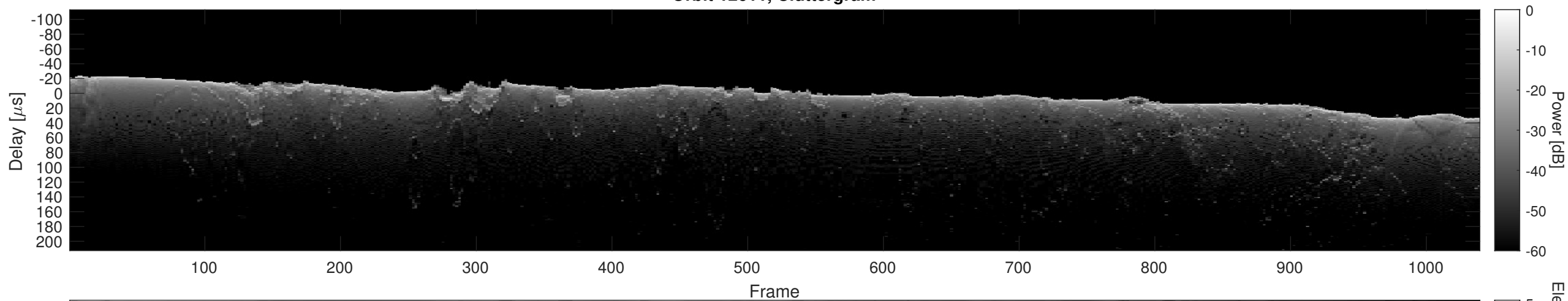
Orbit 12611, Cluttergram
