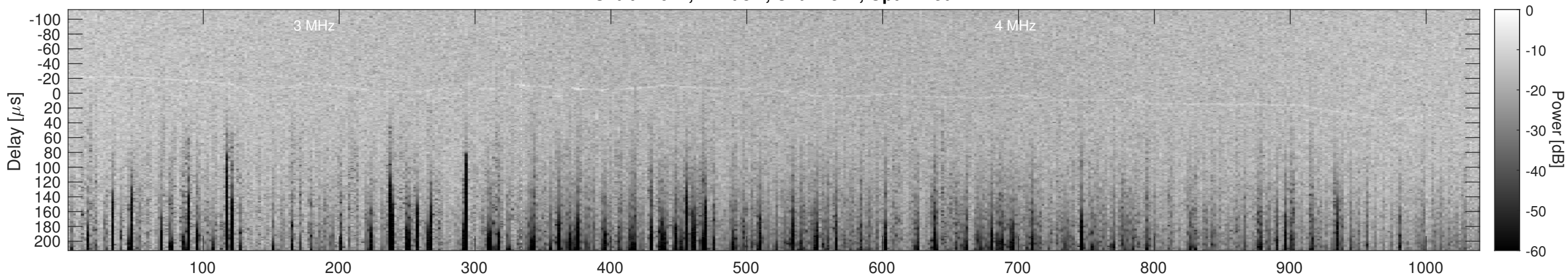
Orbit 12611, Cluttergram
