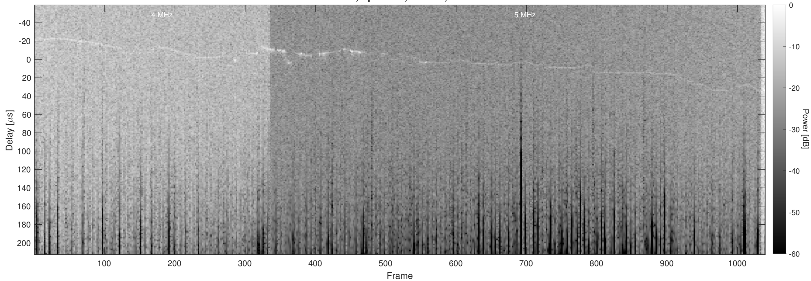
Orbit 12611, Optimized, Window, Channel 2
