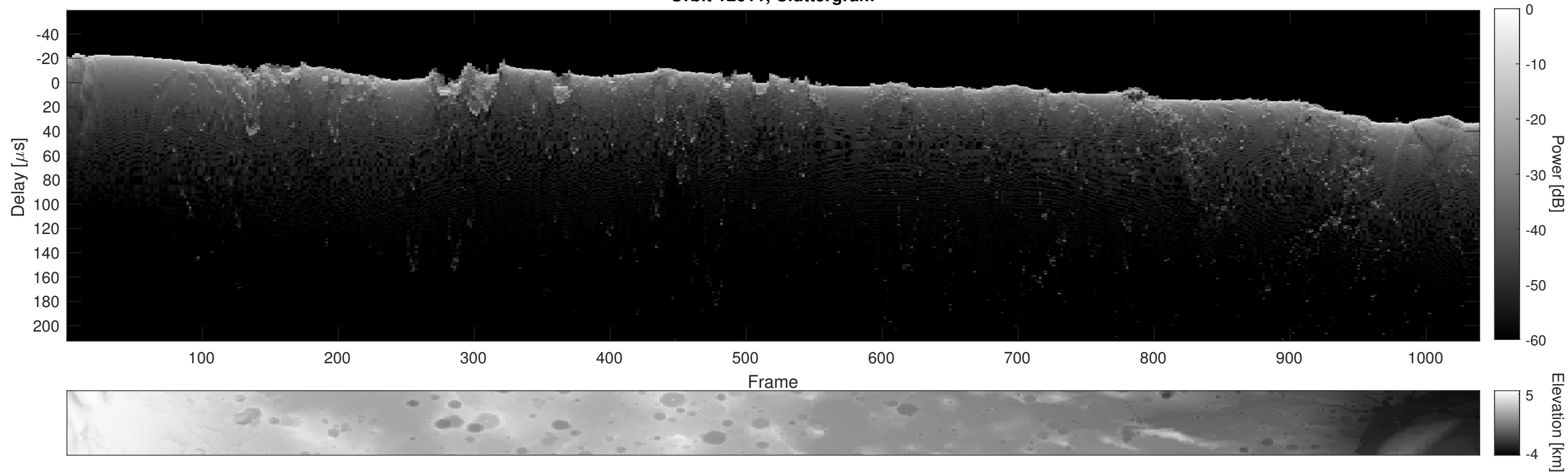
Orbit 12611, Cluttergram
