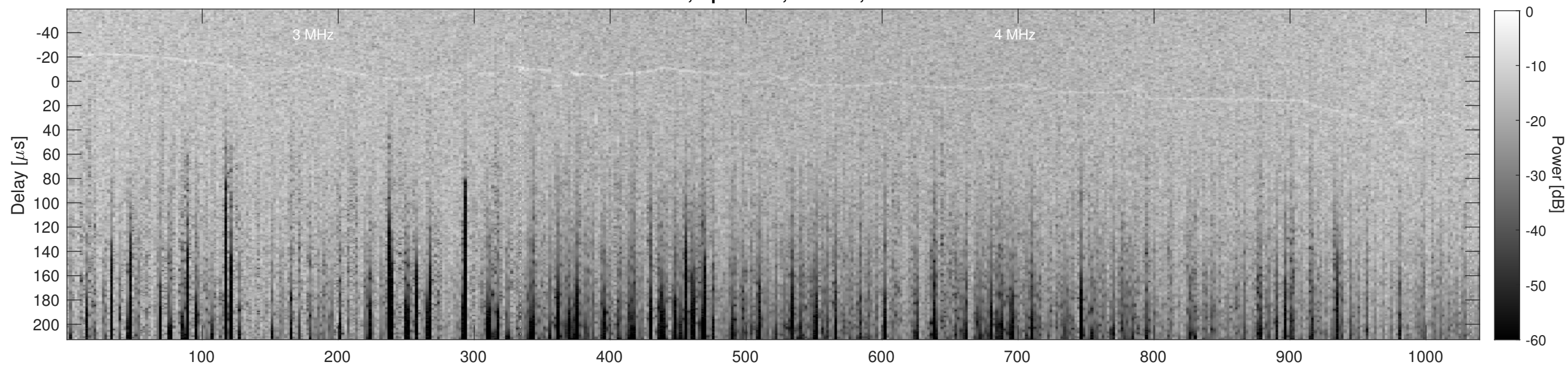
Orbit 12611, Cluttergram
