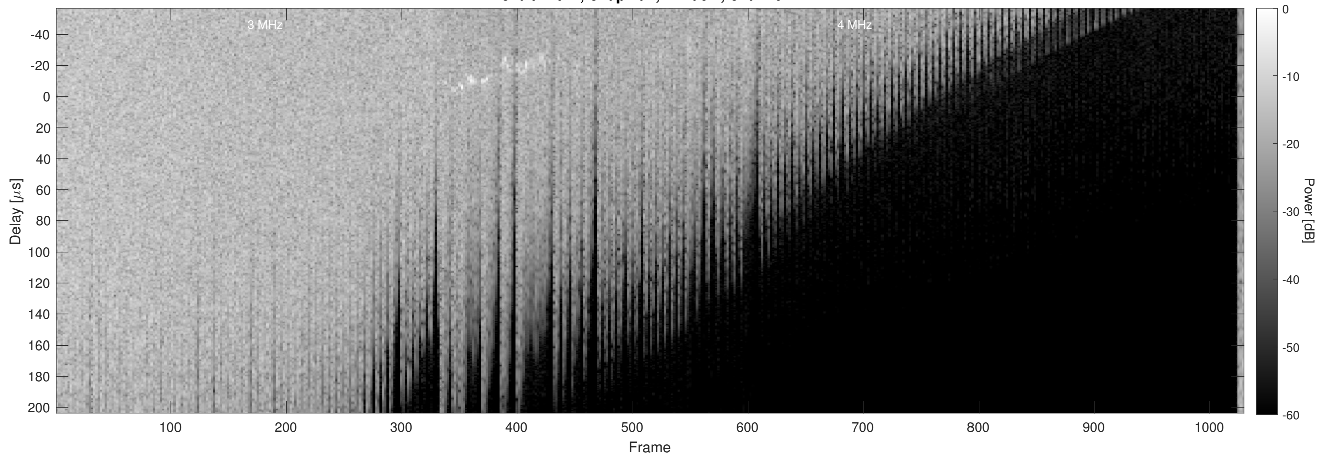
Orbit 12612, Chapman, Window, Channel 2
