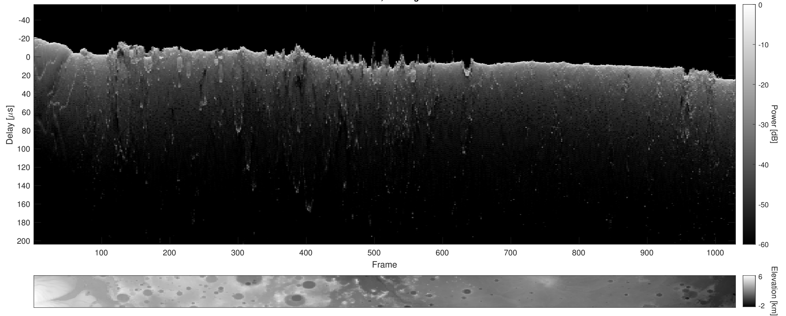
Orbit 12612, Cluttergram
