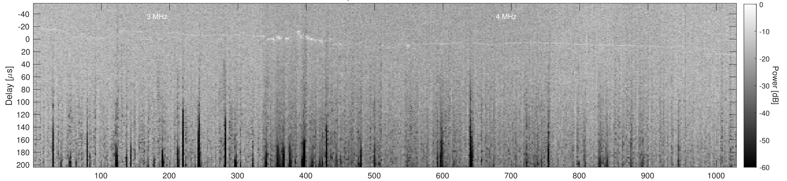
Orbit 12612, Cluttergram
