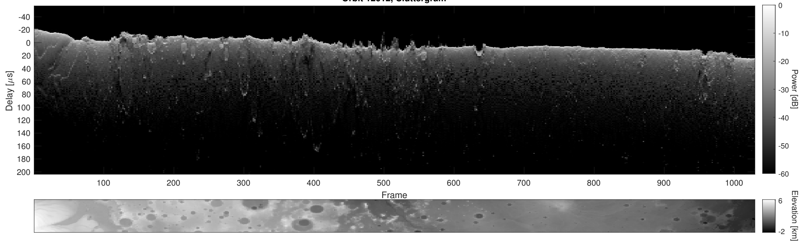
Orbit 12612, Cluttergram
