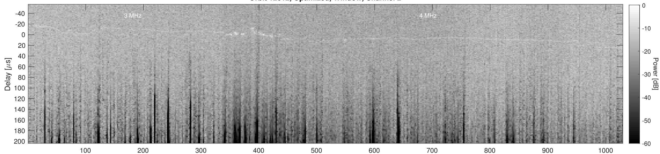
Orbit 12612, Cluttergram
