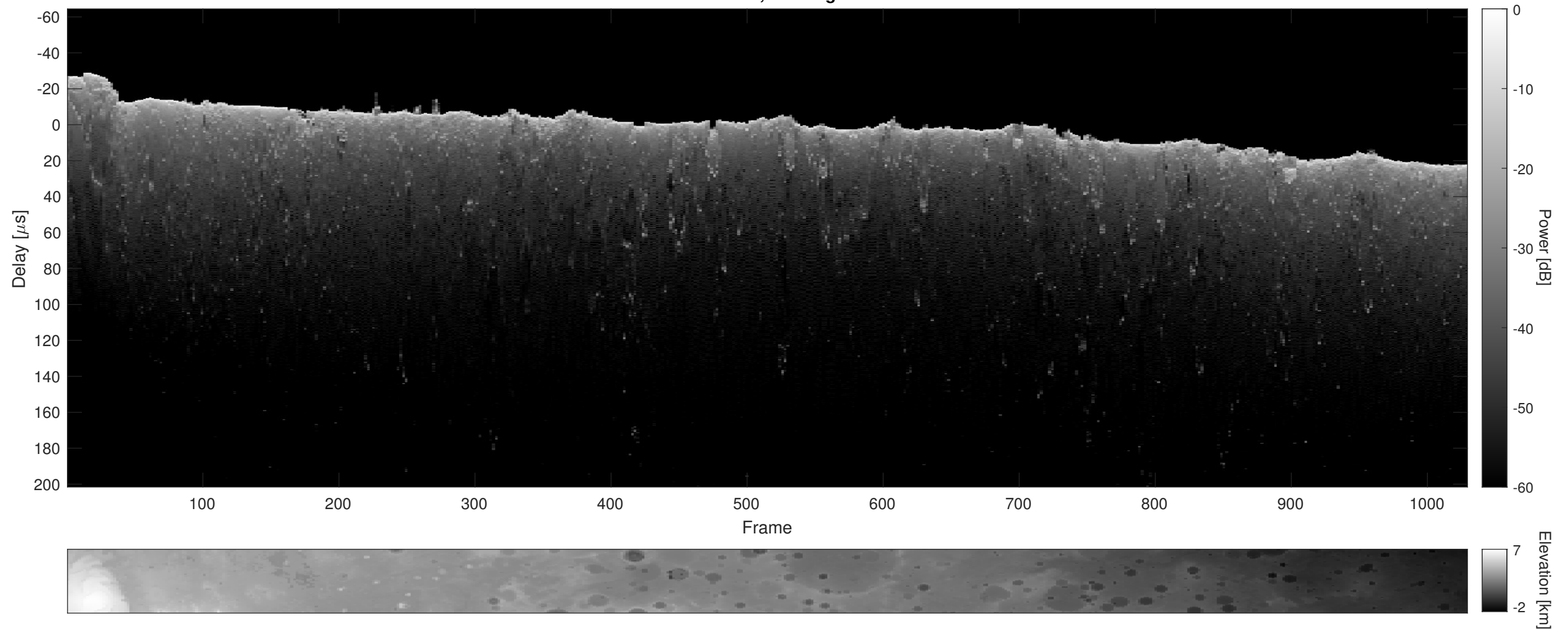
Orbit 12613, Cluttergram
