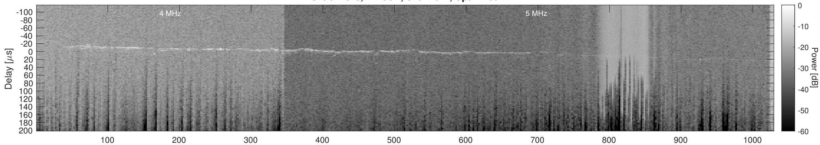
Orbit 12613, Cluttergram
