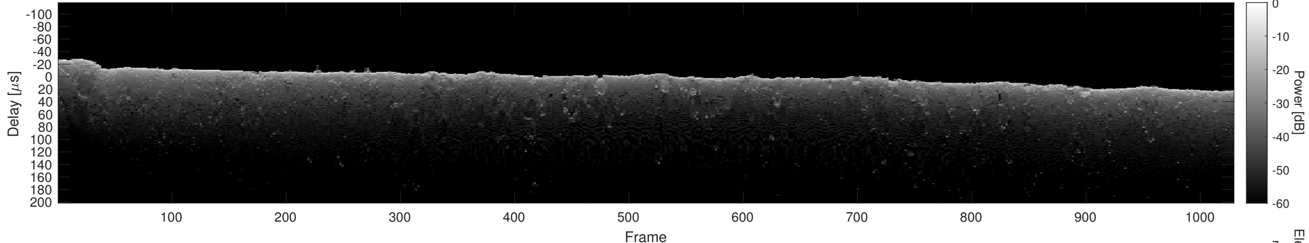
Orbit 12613, Cluttergram
