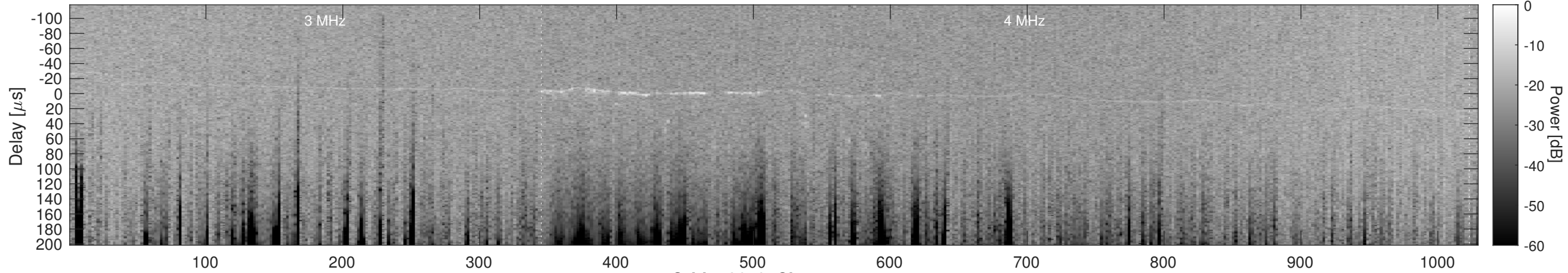
Orbit 12613, Cluttergram
