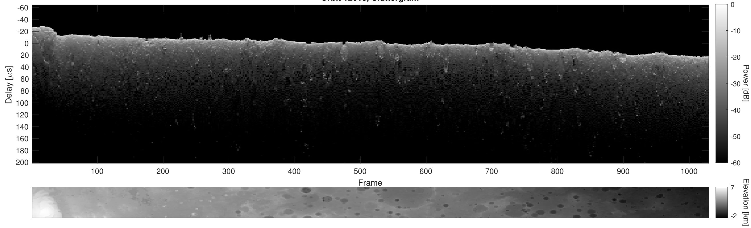
Orbit 12613, Cluttergram
