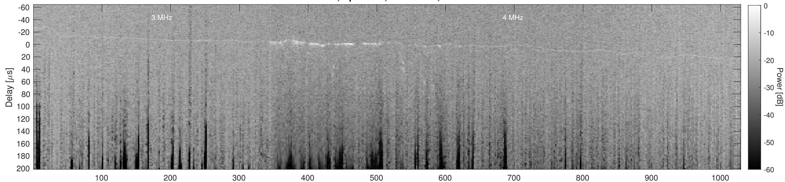
Orbit 12613, Cluttergram
